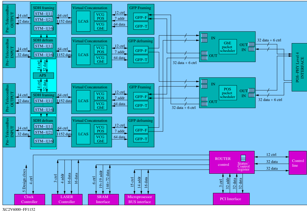
Figure 7.2: The block design for the larger FPGA in the OAN prototype.
