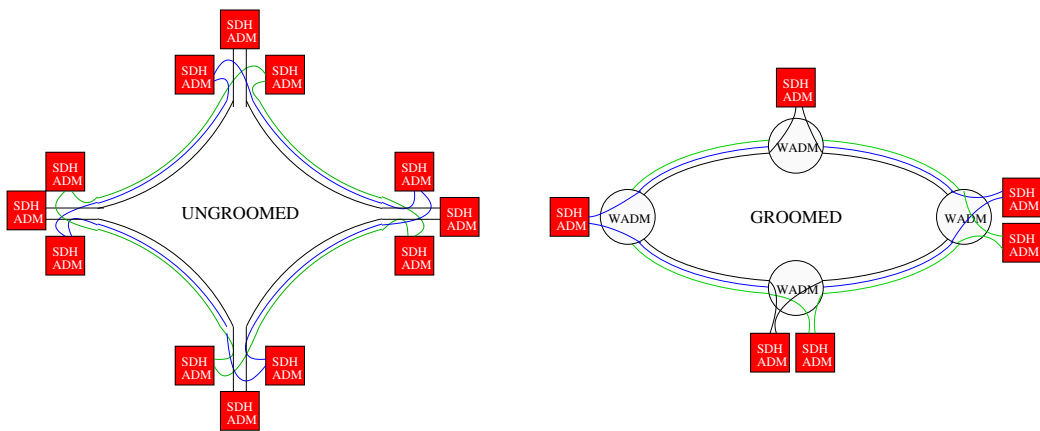
Figure 2.7: Traffic grooming in WDM networks.
