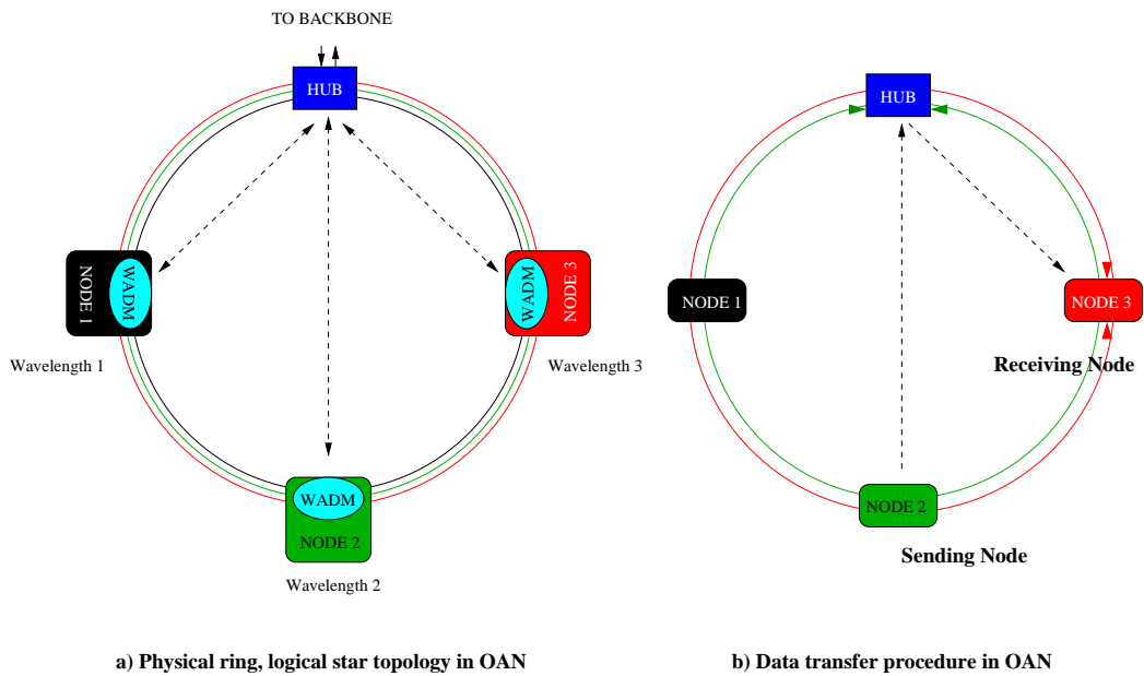
Figure 4.3: The network structure and data transmission process in the OAN test network prototype.
