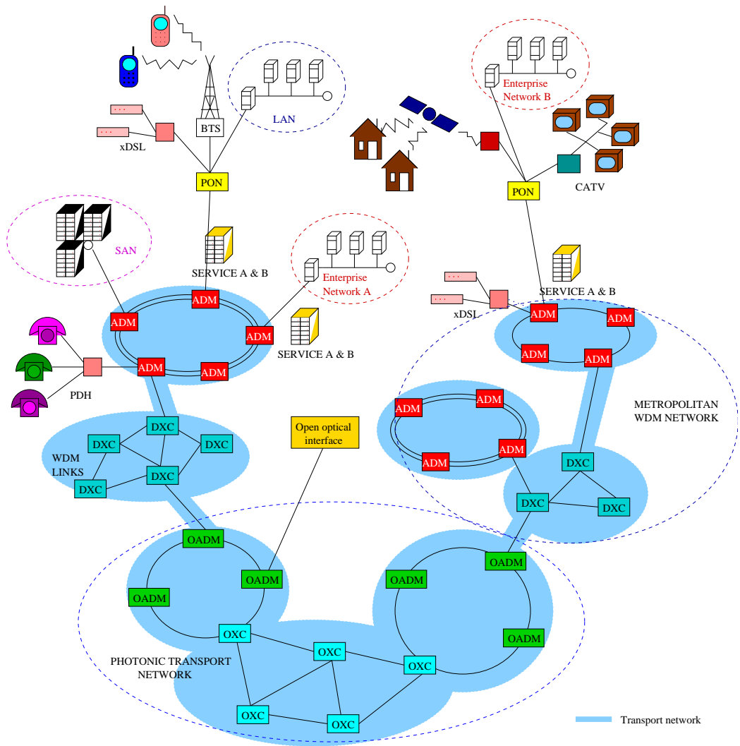
Figure 3.1: The structure of the future communication network.
