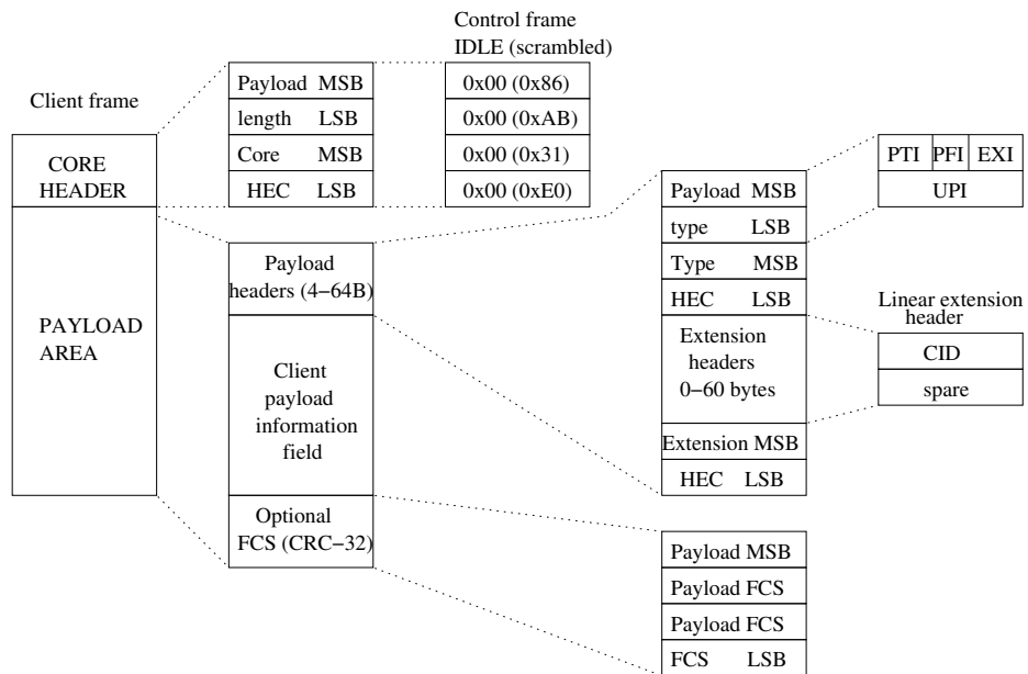
Figure 7.11: The structure of the GFP frame.
