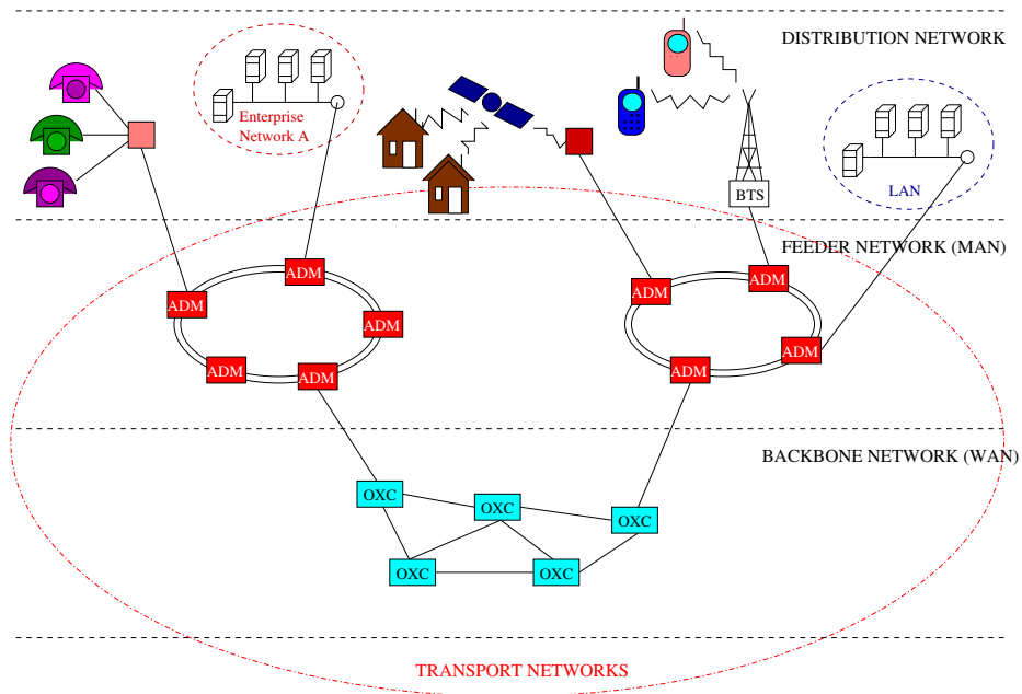
Figure 2.5: The definition of transport network.
