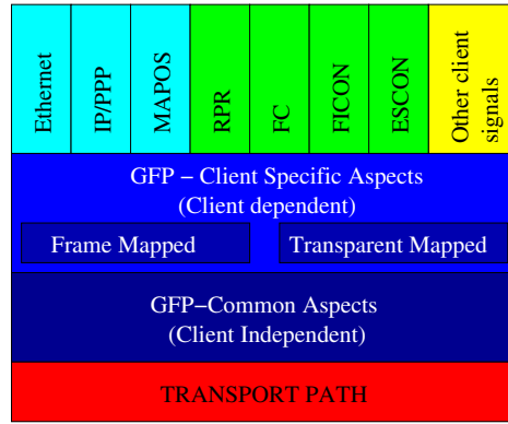
Figure 3.4: Functional model of GFP, adopted from [HVSZ02].
