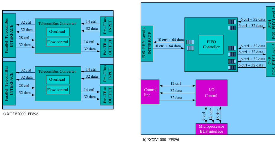
Figure 7.3: The block designs for the smaller FPGA in the router card (a) and for the FPGA in the interface-card (b).
