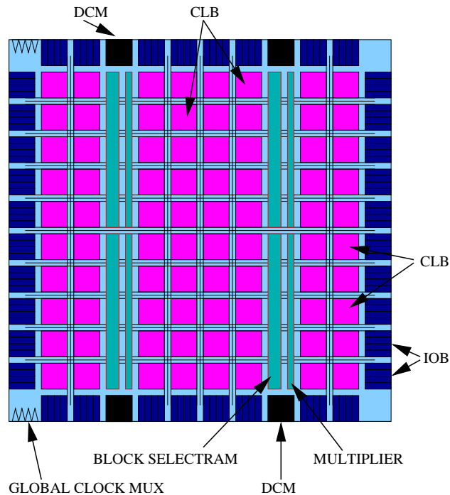
Figure 6.1: Virtex-II FPGA structure, adopted from [Inc00c].
