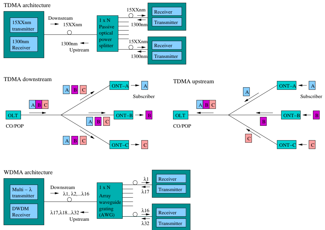
Figure 3.2: The architecture and principle of TDMA and WDMA PONs, adopted from [Com01].
