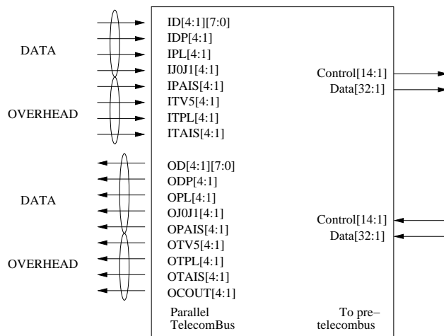
Figure 7.15: The signals in the parallel TelecomBus interface, adopted and modified from [Inc01c].
