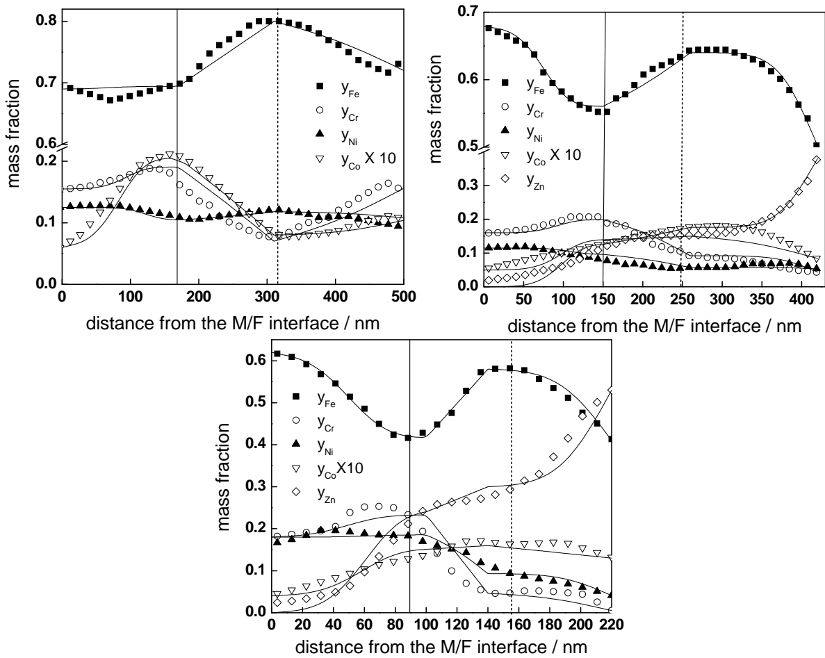
Fig. 34 Experimental (points) and calculated (solid lines) depth profiles of the mass fractions of Fe, Cr, Ni, Co and Zn in the films formed on AISI 316 for 1000 h in simulated BWR water without Zn (above left), with 10 ppb Zn (above right) and 50 ppb Zn (below). The inner layer / outer layer and outer layer / deposited layer boundaries indicated with a vertical line. Data taken from Ref. 59.
