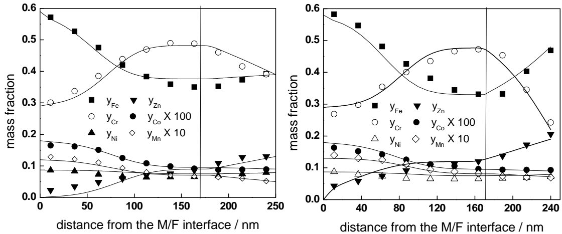
Fig. 9 Experimental (points) and calculated (solid lines) depth profiles of the mass fractions of Fe, Cr, Ni, Co, Mn and Zn in the films formed on AISI 304 after the exposure to ca. 100 and 300 EFPD (125 and 336 days) in the Halden Reactor, PWR coolant conditions. The inner layer / outer layer boundary indicated with a vertical line. Experimental data taken from Refs 29-31.
