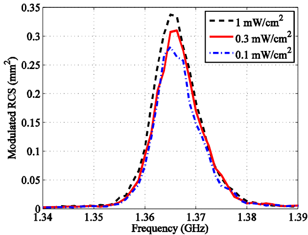
Fig. 4. The measured modulated radar cross section (RCS) of the transponder. The curves are for different irradiance levels.
