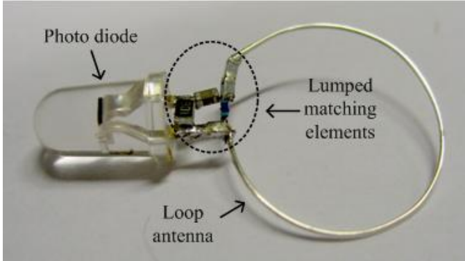
Fig. 3. A photograph of the photo-activated microwave transponder.
