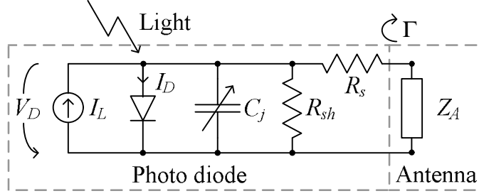
Fig. 1. An electrical equivalent circuit of the wireless photo detector.
