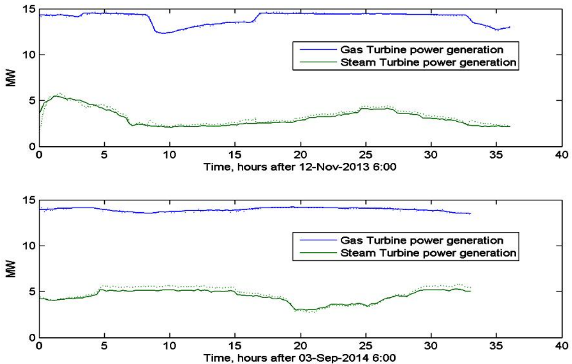
Figure 4: Calculated and Measured Electric Power Production Rates (solid = measured, dotted = simulated)
