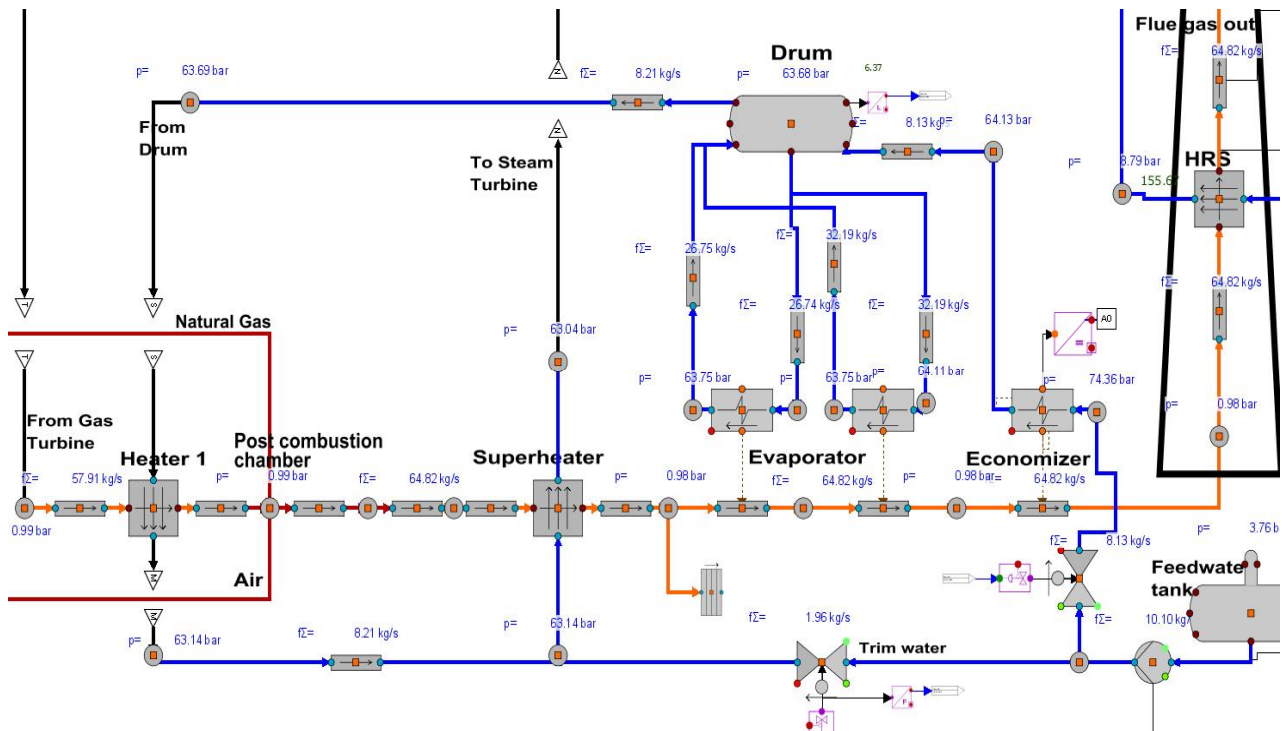
Figure 2: The Flue Gas Path as Shown by Apros
