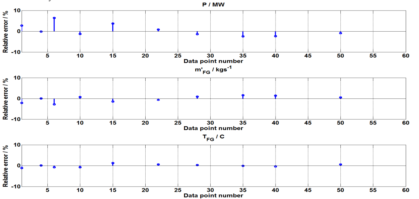
Figure 5: Relative Errors between the Calculated Values and Apros Data at Validation Data Points (%)
