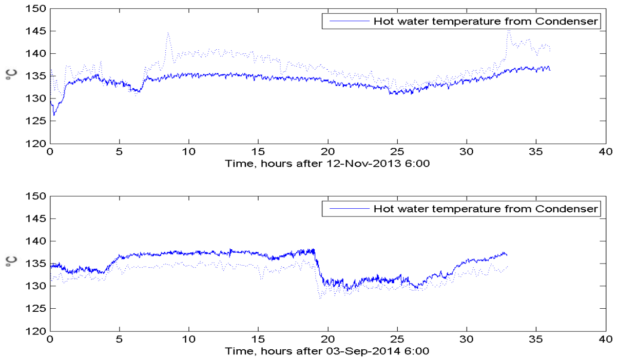
Figure 3: Calculated and Measured Temperatures of the Hot Water Flow from the Steam Condenser (solid = measured, dotted = simulated)
