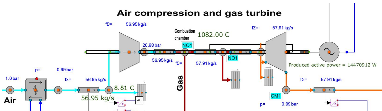
Figure 1: The Gas Turbine Process as Apros Displays it
