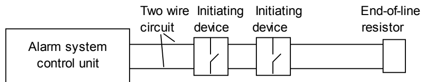
Figure 1. Principal structure and components of a stub line (Class B in NFPA 72) fire alarm system (Öystilä 1990).
